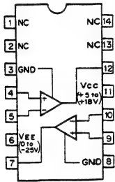
uPC272C (NEC) uPC319C (NEC) DUAL VOLTAGE COMPARATOR — TOP VIEW —
